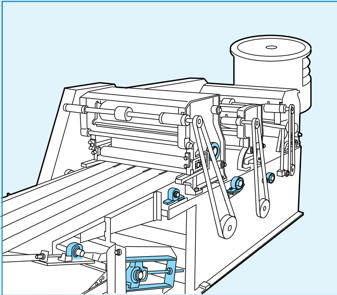
Noodle-making machine
